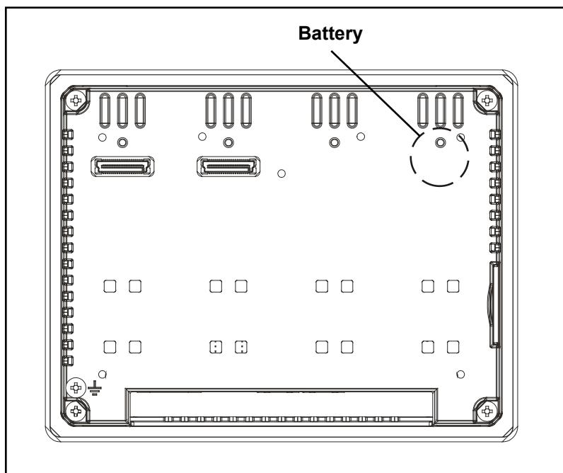
Fig. 7.2: eX707, eX710, eX715, eX721
