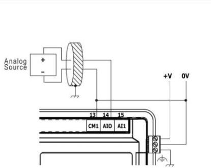
Differential
