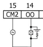
AC Load
