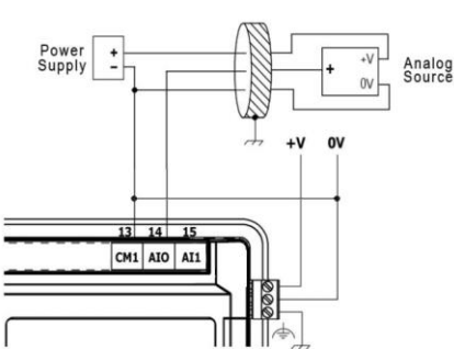
3-wire
