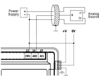
3-wire
