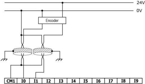
High Speed Input wiring, sink
