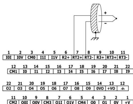
Thermocouple
