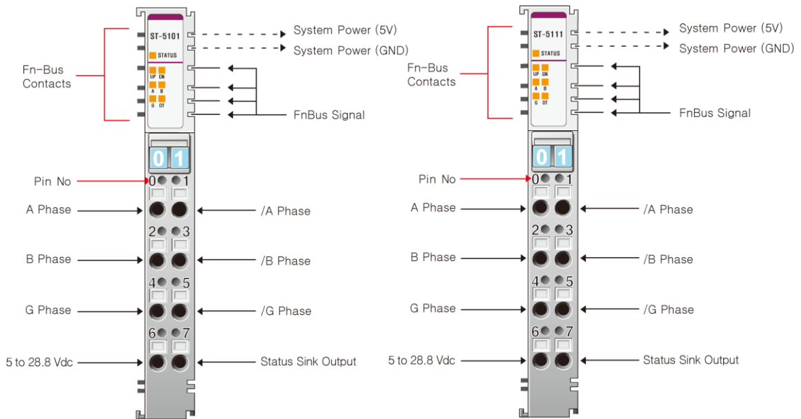
(1) Open Collector
