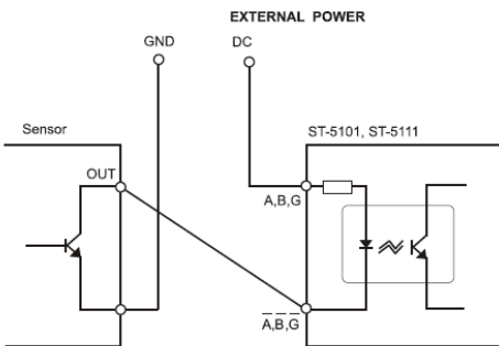
(1) Open Collector
