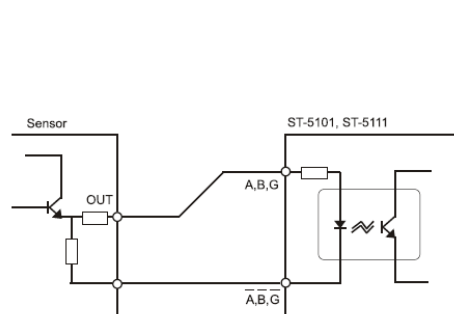
(2) VOLTAGE OUTPUT
