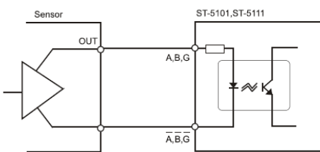
(3) LINE DRIVE
