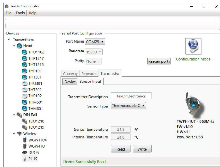
Figure 14 - Sensor input tab in Tekon Configurator software
