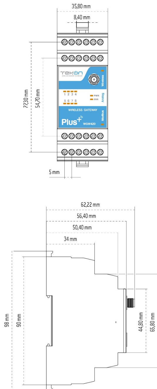
Figure 39 – WGW420 gateway mechanical interface and dimensions
