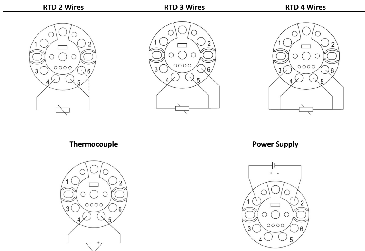
Figure 15 - TWPH-1UT wire connections
