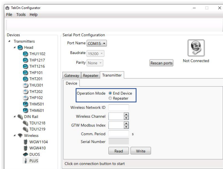
Figure 47 - Transmitter operation mode configuration in Tekon Configurator
