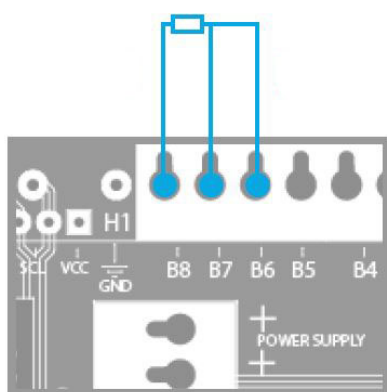
Figure 20 - PT100 connection
