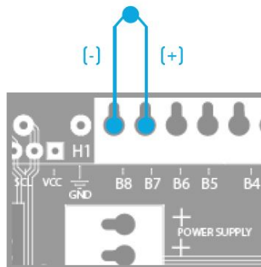
Figure 21 - Thermocouple connection
