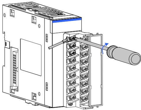
Figure 6 Connecting cable to terminal block
