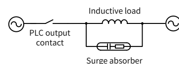
Figure 9 AC circuit contact protection when using inductive load
