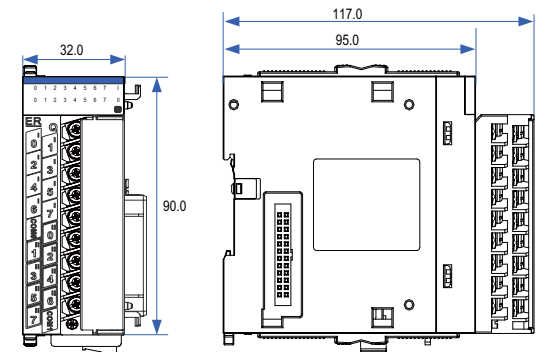
Figure 4 Mounting dimensions (in mm)
