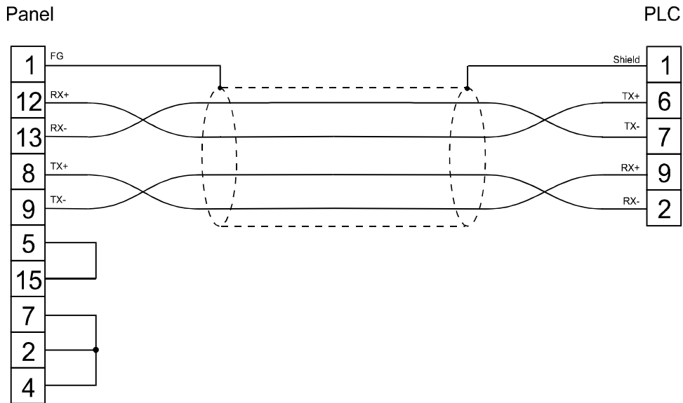
figure 1. Cable diagram
