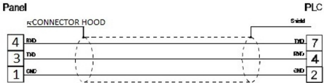
figure 1. Cable diagram
