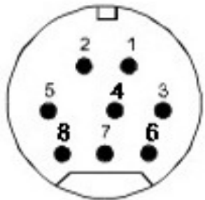
figure 2. Connector front view (pin side)
