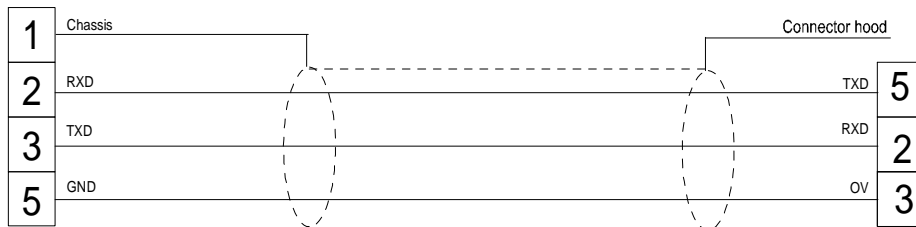
Figure 1. Cable diagram
