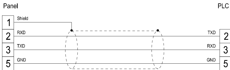
Figure 1. Cable diagram
