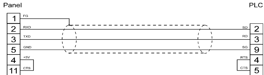
figure 1. Cable diagram
