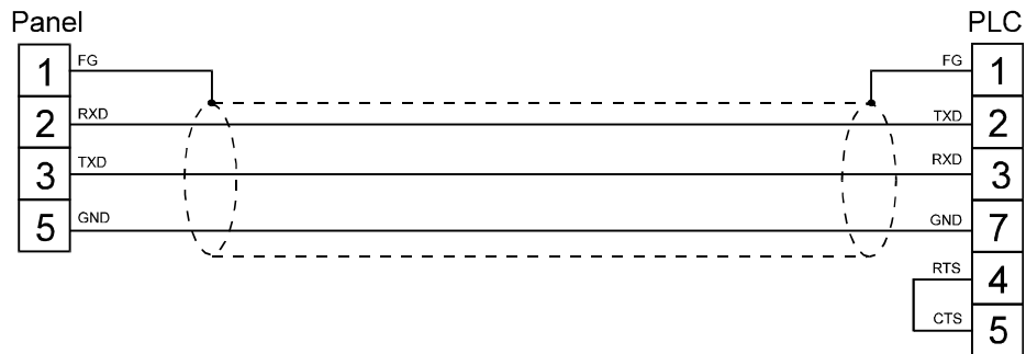
figure 1. Cable diagram
