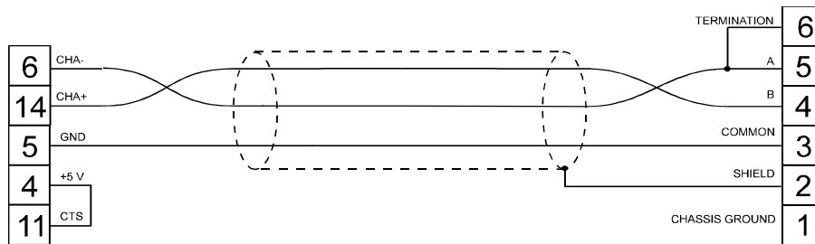
figure 1. Cable diagram
