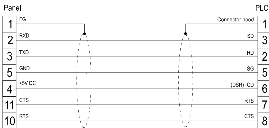
Figure 1. Cable diagram
