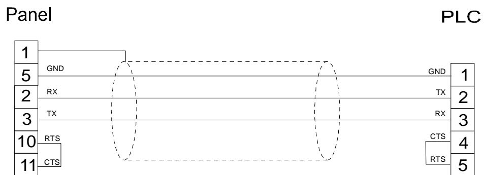
Figure 1. Cable diagram
