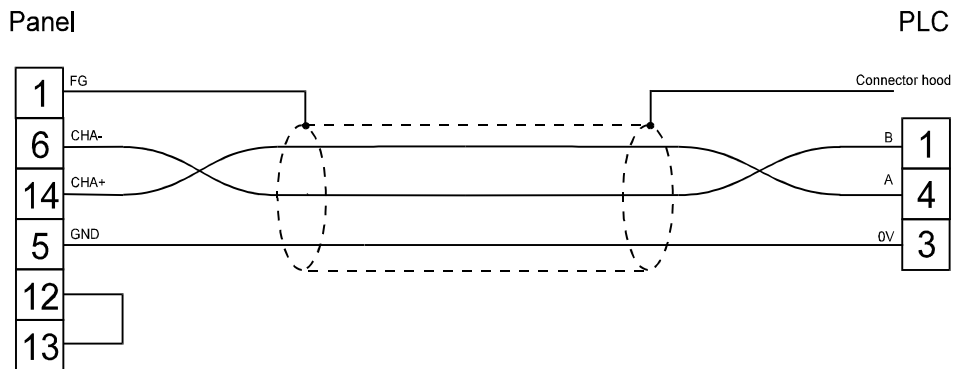
figure 1. Cable diagram
