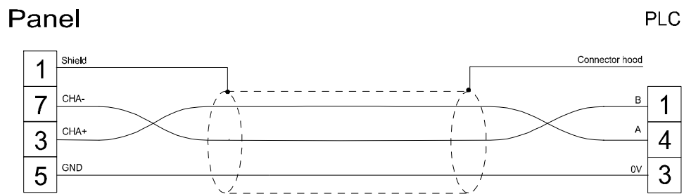
figure 1. Cable diagram
