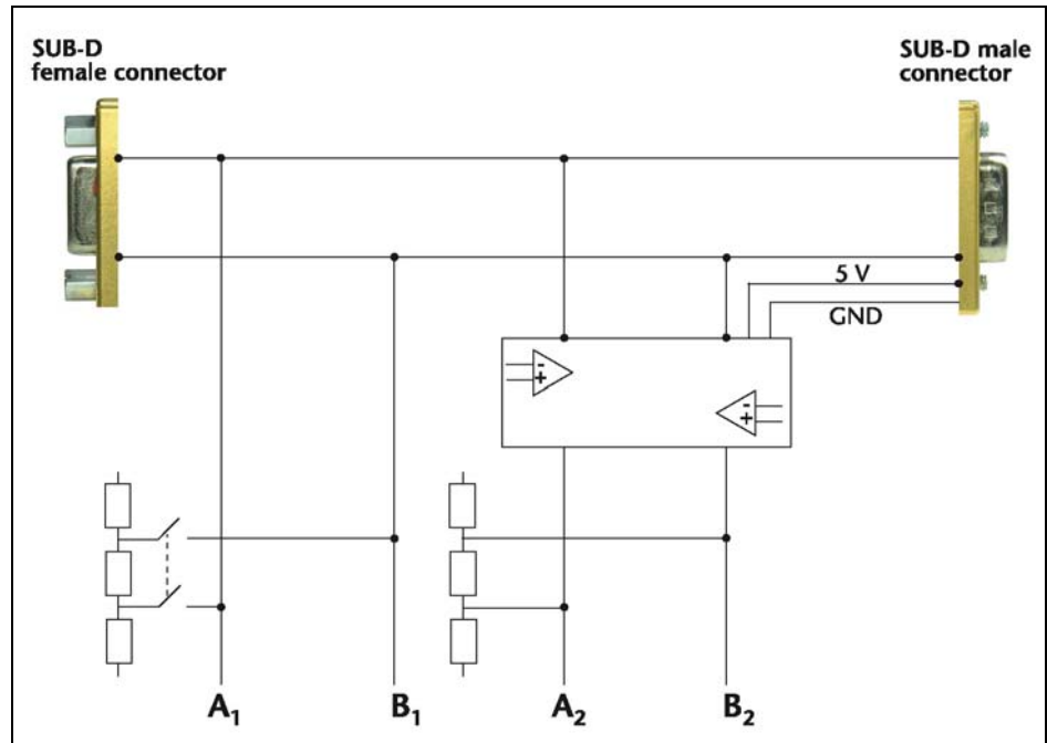
Fig. 3-2: Block diagram of the repeater
