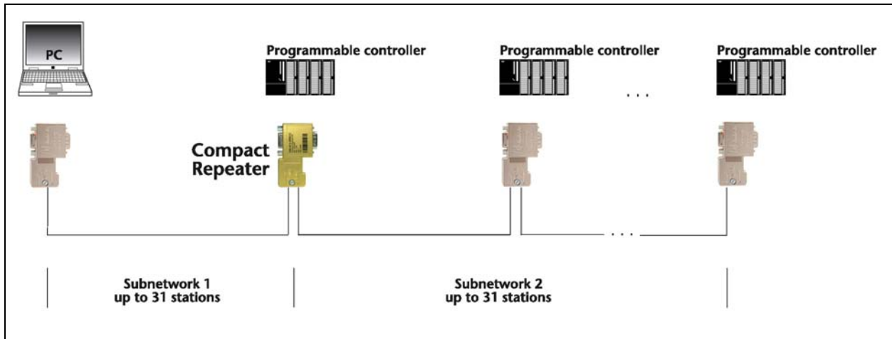
Fig. 3-3: Application example of a long bus line
